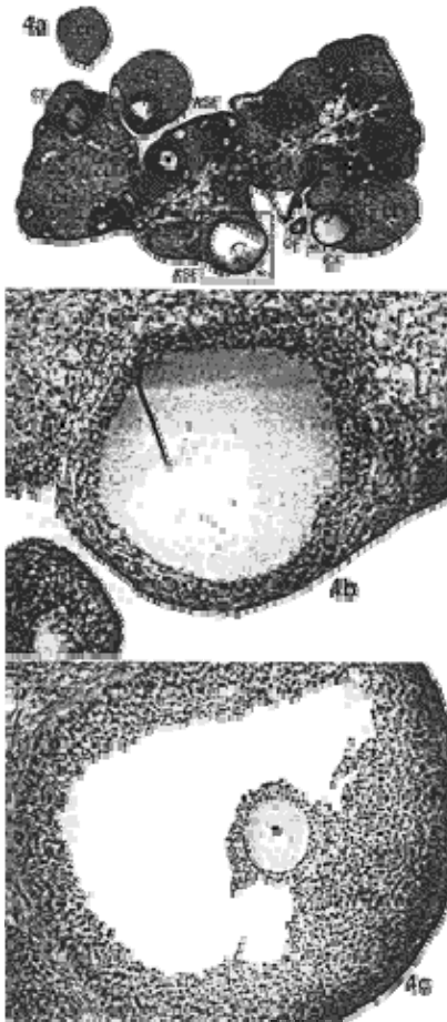
FIG. 4. a) Section of an ovary from a rat injected with 4 mg EV in 0.2 ml oil and sacrificed on Day 30. In total, seven corpora lutea marked with CL three cystic follicles (CF) marked with CF, and two atretic secondary follicles marked with ASF are seen. One cystic follicle (b) and one atretic secondary follicle are framed (c). Magnification x2.5: Section stained with hematoxylin-eosin. b) Cystic degenerating follicle showing a thin granulosa layer and debris in follicular fluid. Magnification x20. c) An atretic secondary follicle with detachment of the oocyte from the cumulus mass of pyknotic granulosa cells. Magnification x20.
